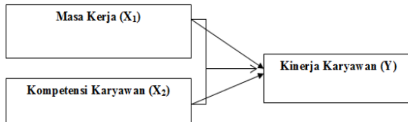
Gambar 1: Model Hipotesis
