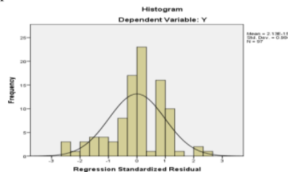
Picture 2. Result Normality test
